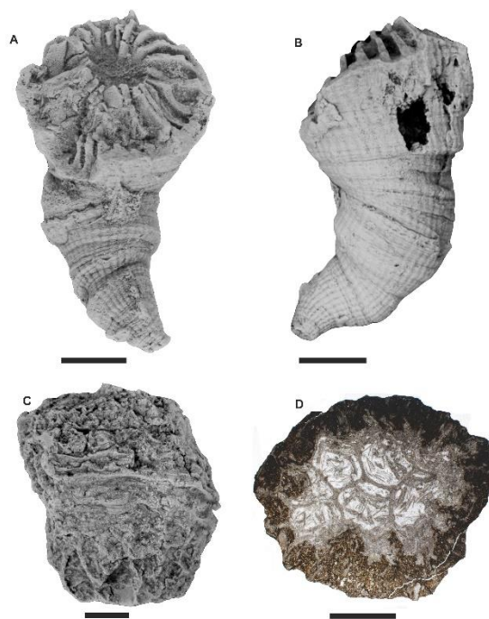
Fig. 3. Impact of diagenesis on two coral specimens: A–B. External views of an antiphyllid rugose coral specimen ( Rotiphyllum? sp.), displaying well-preserved epithecal wall showcasing septal furrows, growth lines, constrictions, and rejuvenations. Additionally, apparently well-preserved septa are observed at the base of the eroded calyx. Despite the apparent preservation of outer features, internal dolomitization and ferrugination have resulted in hollow portions within the corallite (B). C–D. A tabulate coral ( Michelinia sp.), showing relatively well-preserved colony morphology (C) however, internal structures exhibit significant damage (D).
